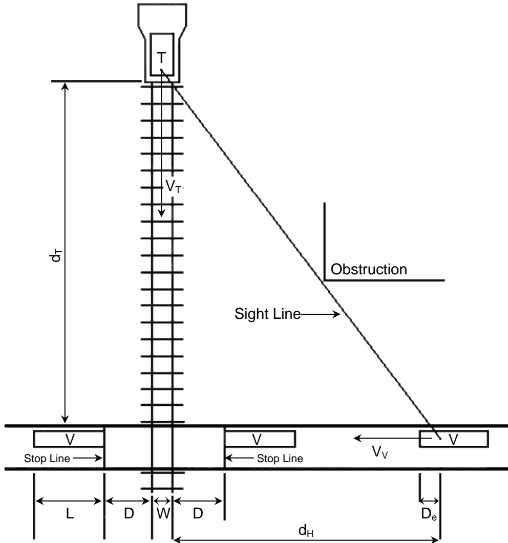
CASE A: Moving Vehicle to Safely Cross or Stop at Railroad Crossing
