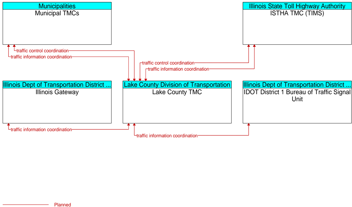
Figure A3-34: Lake County Traffic Management Center- Roadside Interfaces (ID 31)
