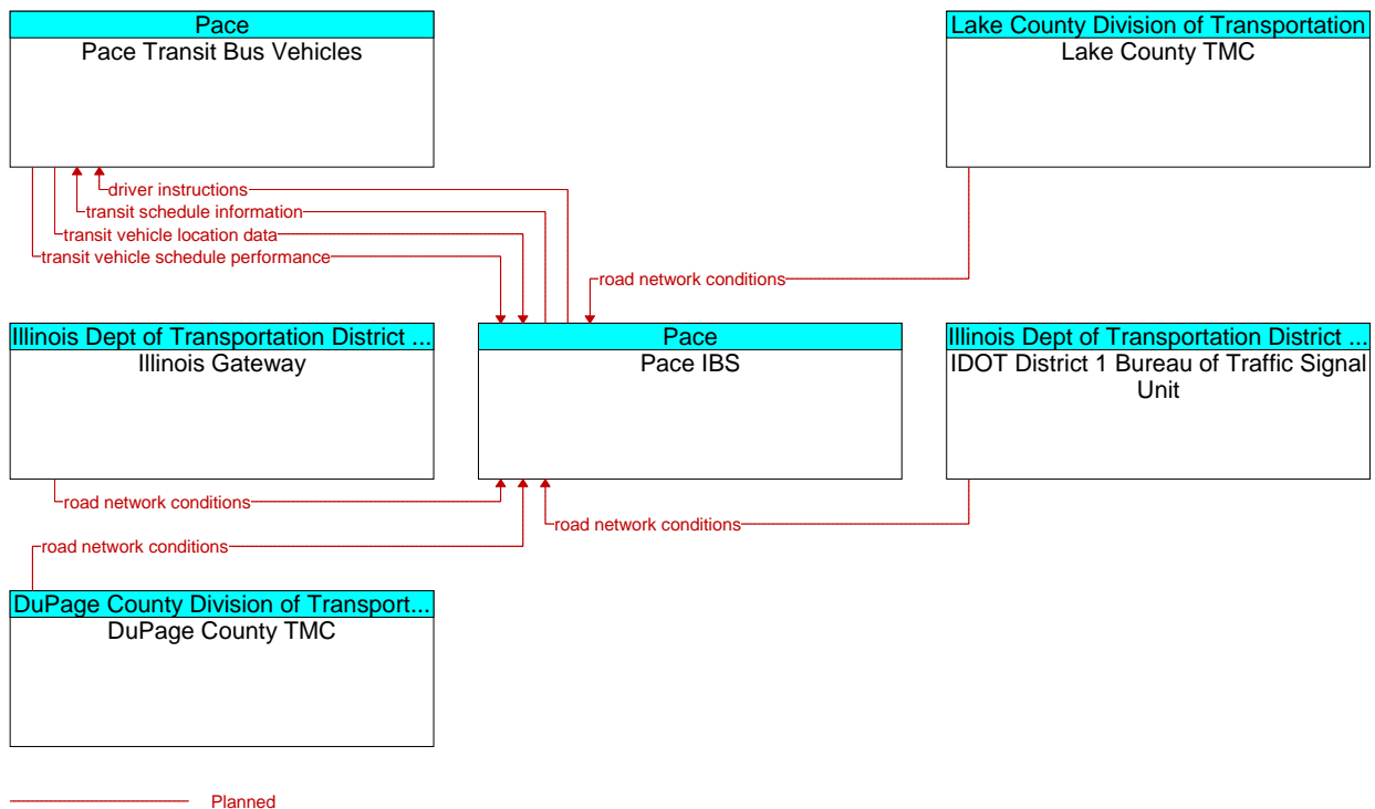
Figure A3-103: Pace Transit Operations Decision Support System (ID 97)
