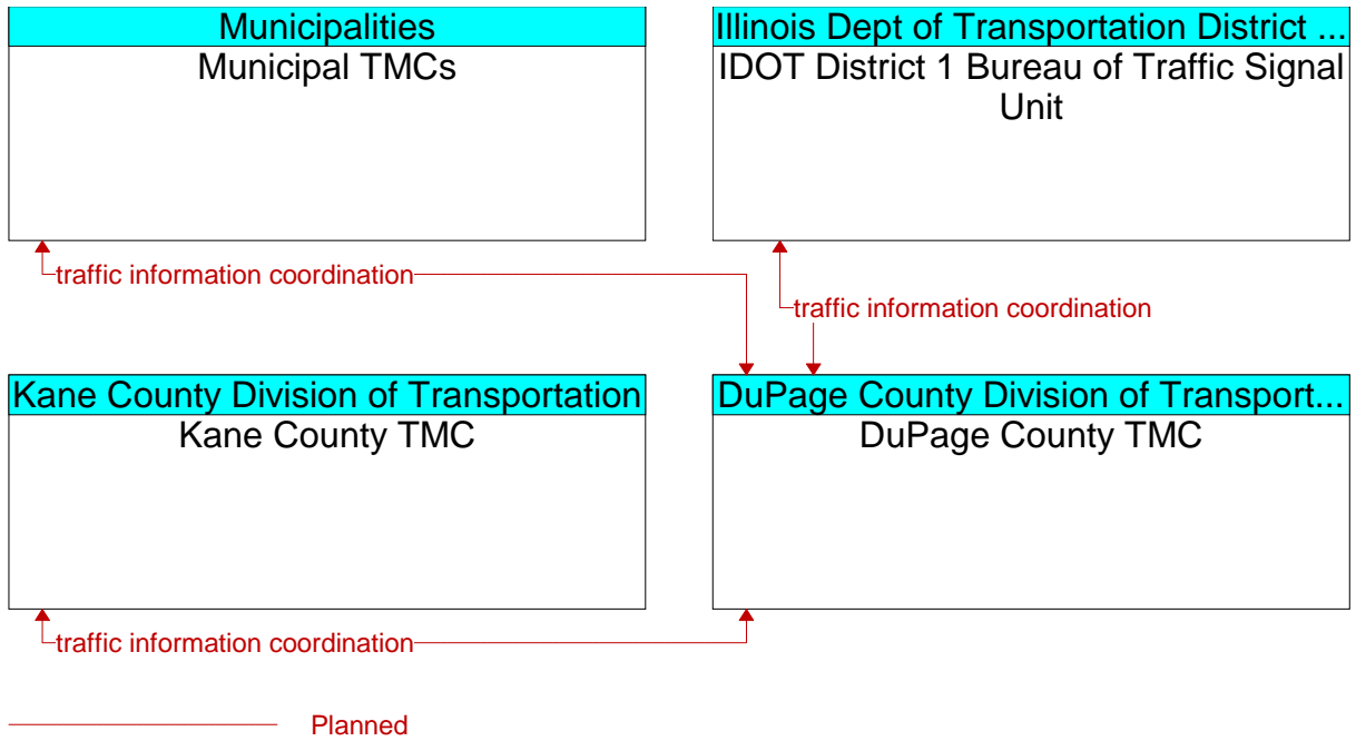
Figure A3-28: Interagency Signal Coordination- DuPage County (ID 27)
