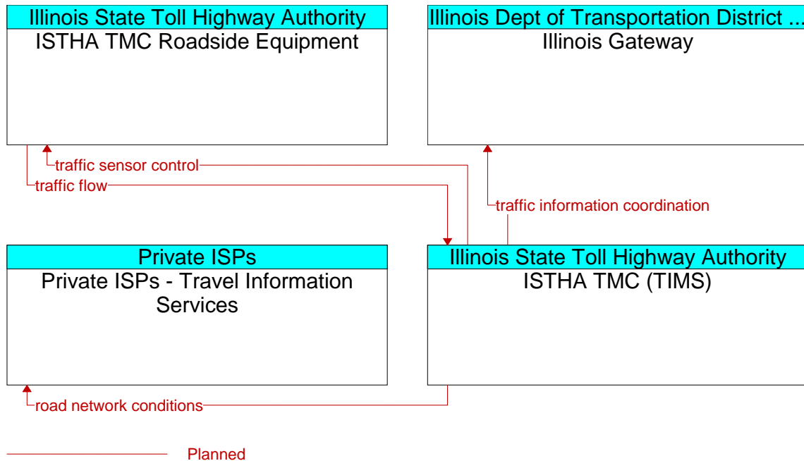
Figure A3-74: ISTHA DMS Deployment (ID 74)
