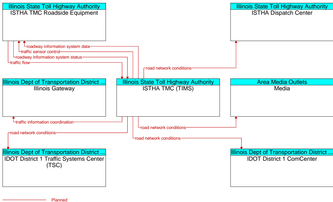
Figure A3-70: ISTHA Portable Queue Detection Systems (ID 70)
