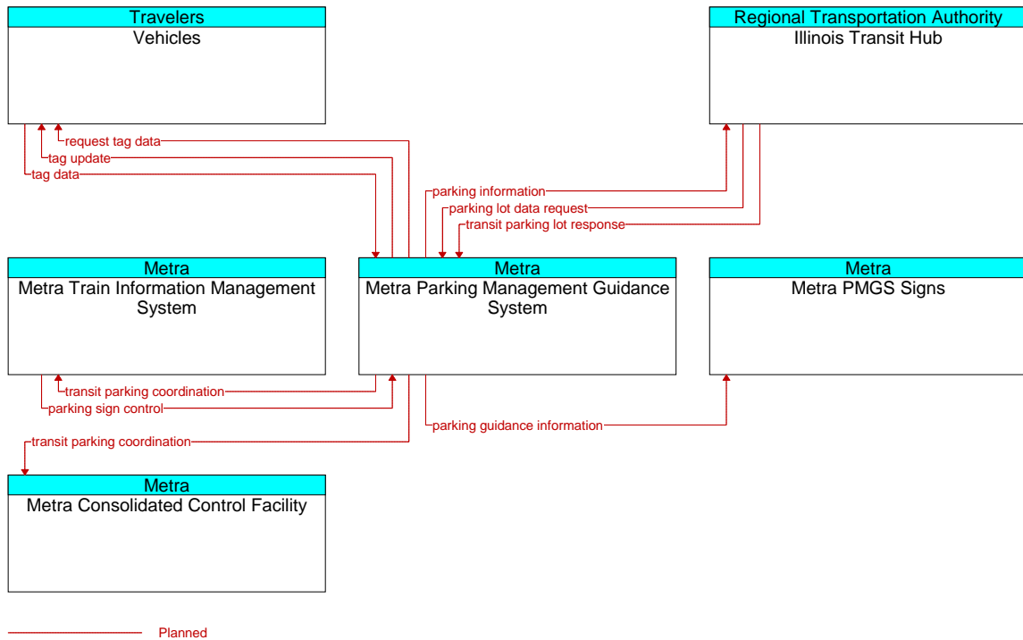
Figure A3-86: RTA Projects: ATIS- Parking Management Guidance Systems (ID 78f)
