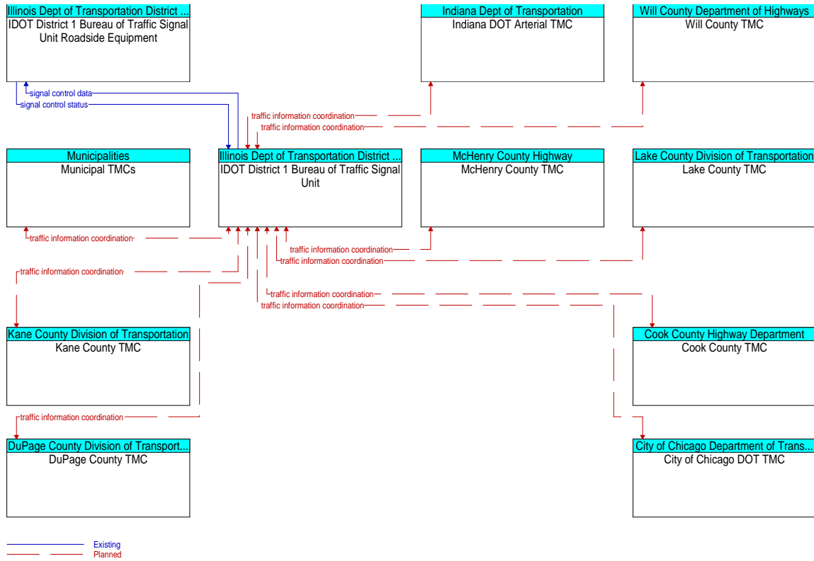
Figure A3-50: Interagency Operations and Signal Coordination (ID 42)
