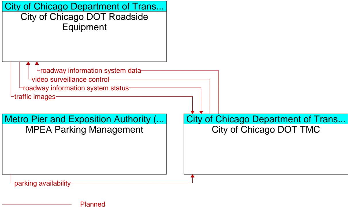
Figure A3-8: Museum Campus Transportation System (Cook/Chicago) (ID 7)
