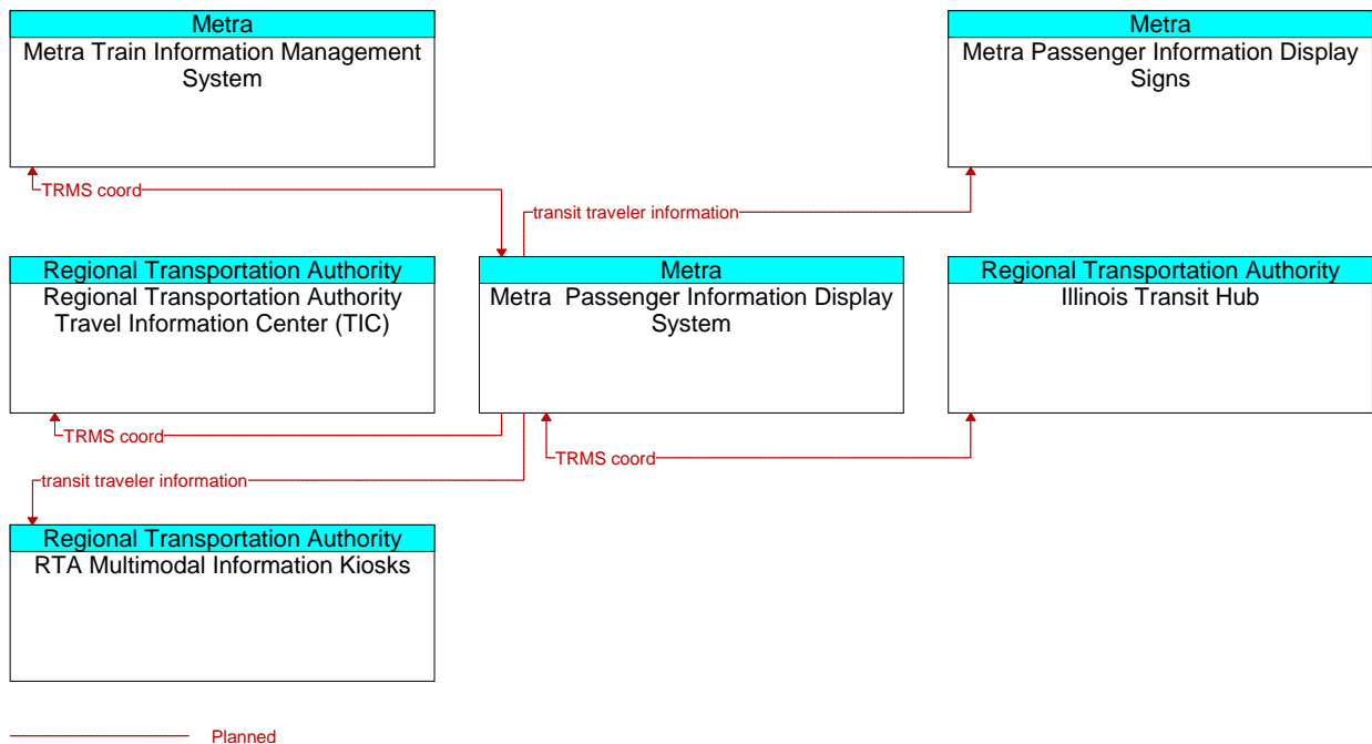
Figure A3-97: PIDS Modernization (ID 90)
