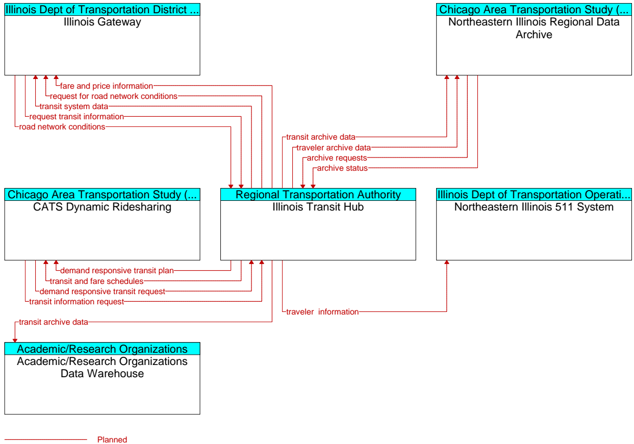
Figure A3-77: Transit Hub: APTS (ID 75)-Regional Transportation System Interfaces
