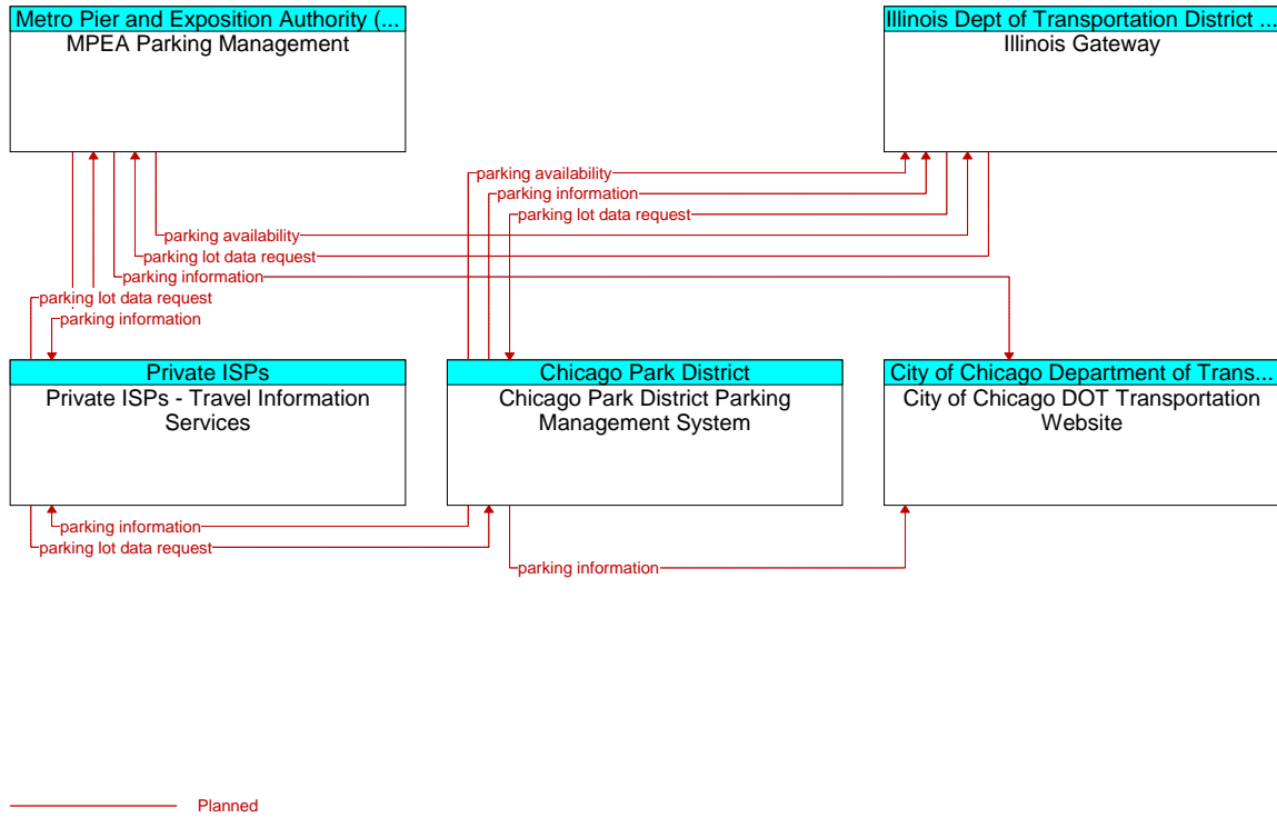
Figure A3-18: Parking Information Projects (ID 18)
