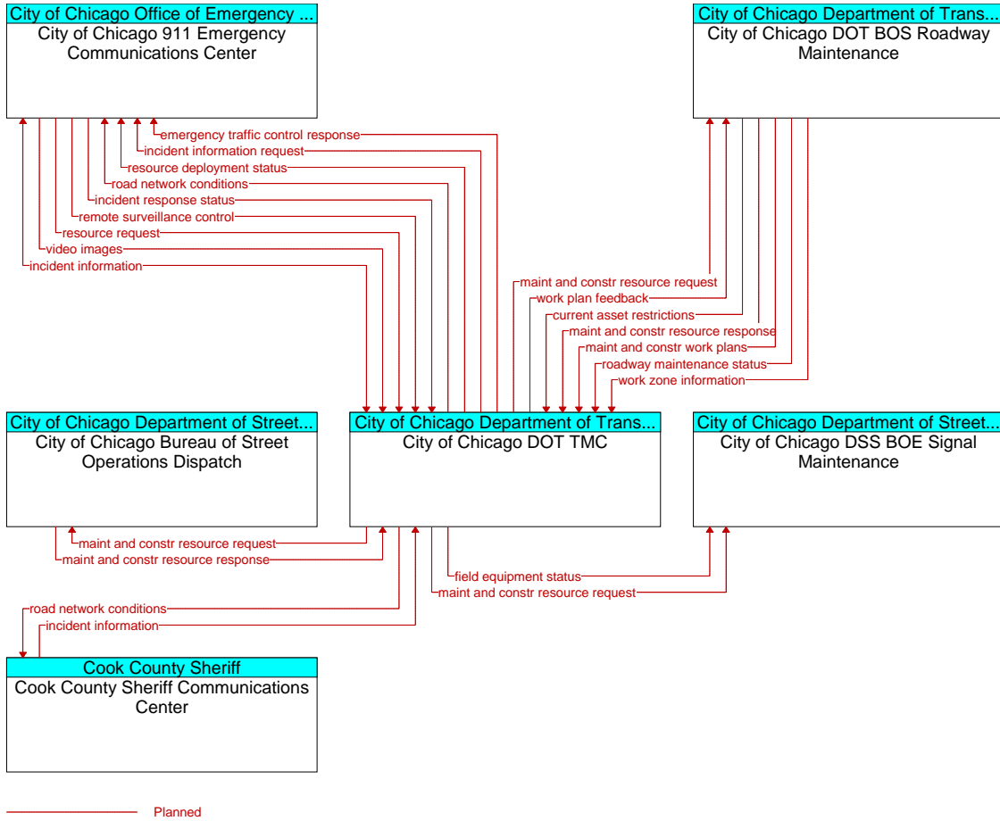
Figure A3-3: Development of Chicago TMC (ID 2)- Emergency and Maintenance Interfaces
