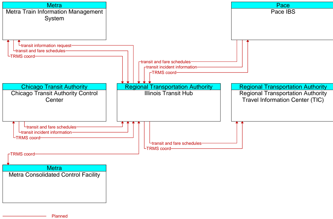
Figure A3-75: Transit Hub: APTS (ID 75)- Primary Service Board Center Interfaces
