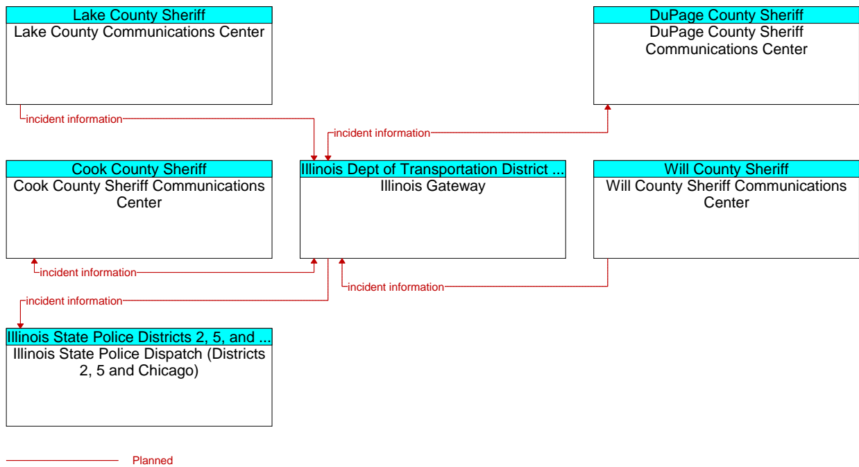
Figure A3-60: GATEWAY Traveler Information System, Phase II (ID 55) - emergency management interfaces
