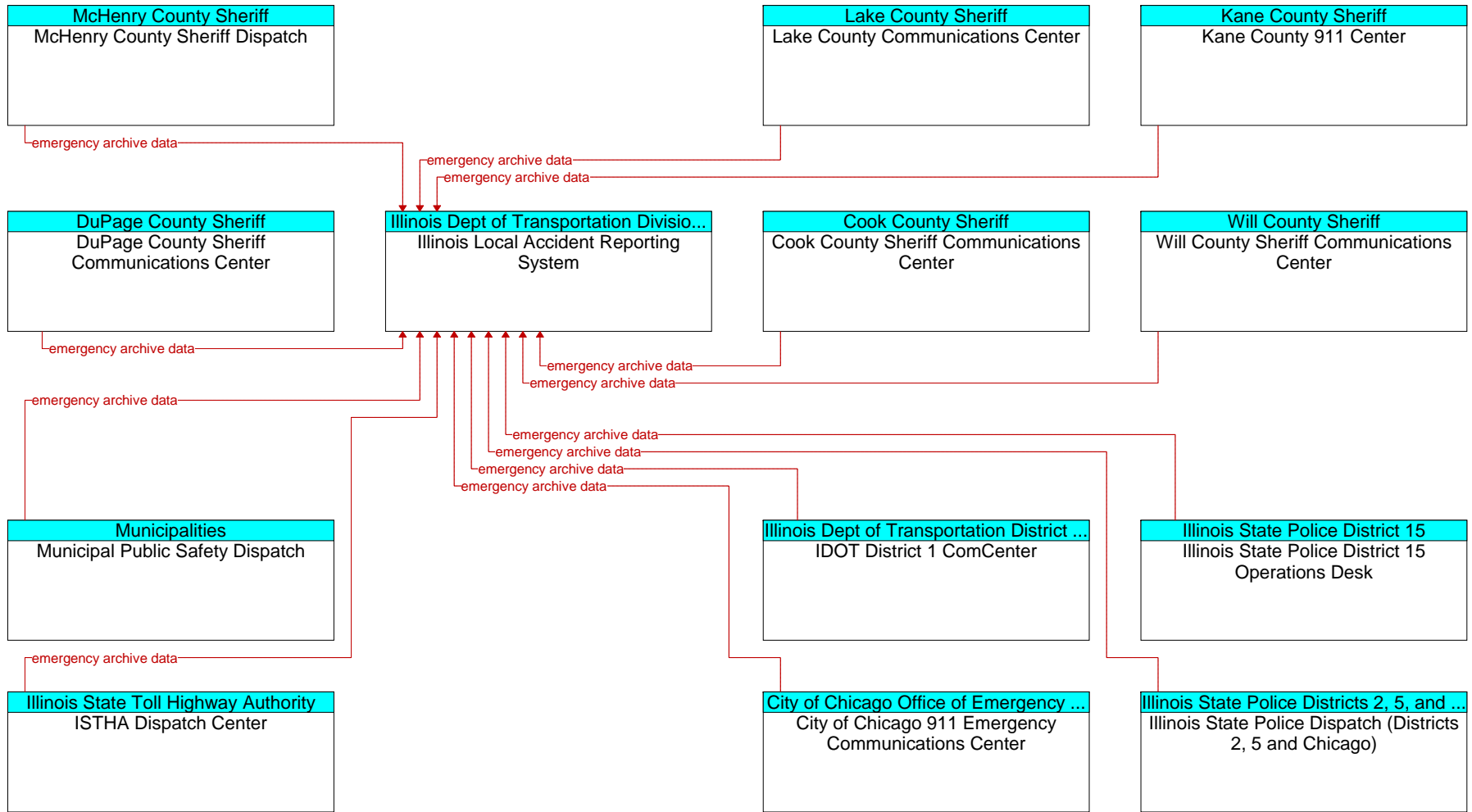
Figure A3-64: Accident Database and Reporting System (ID 59)
