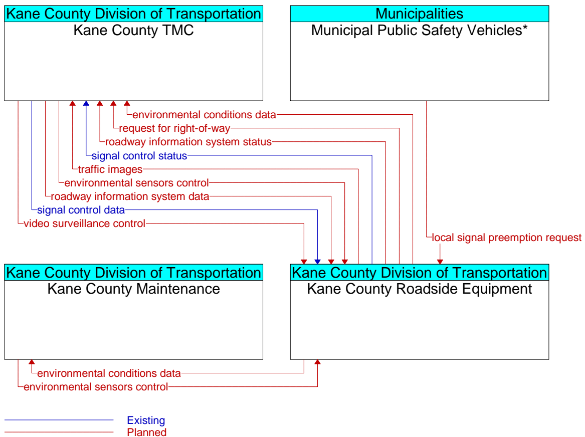
Figure A3-32: Kane County Field Devices (ID 29)
