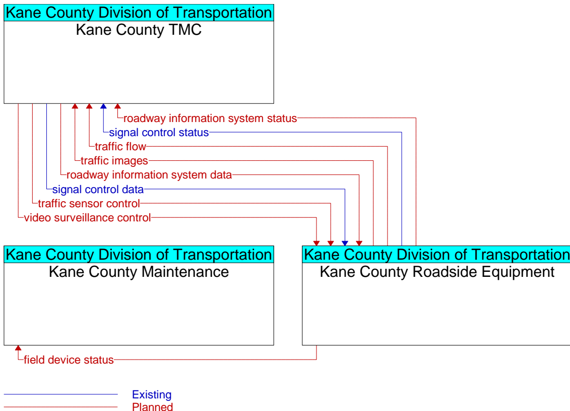
Figure A3-29: Kane County Traffic Management Center-Roadside Interfaces (ID 28)
