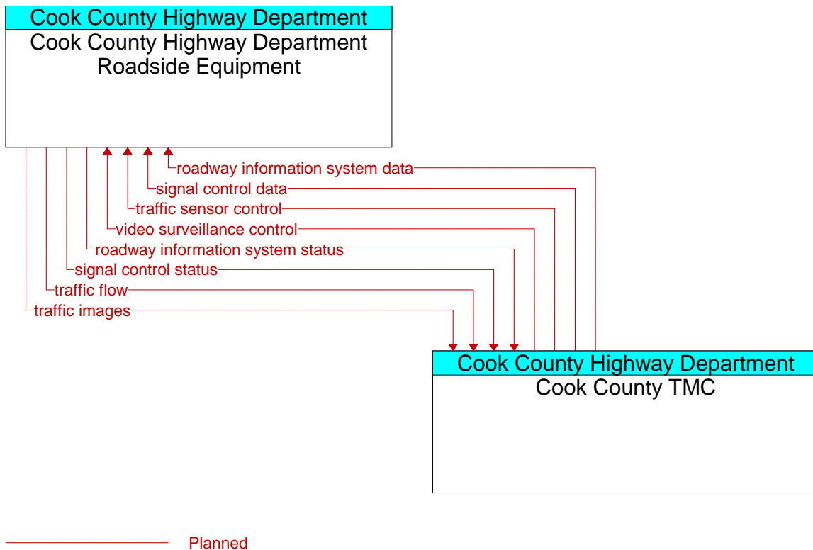
Figure A3-19: Cook County TMC- Roadside Equipment Interfaces
