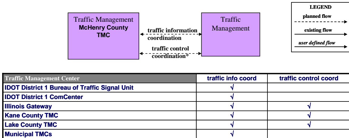
Figure A3-40: McHenry County Traffic Management Center- Traffic Management Interfaces (ID 34)
