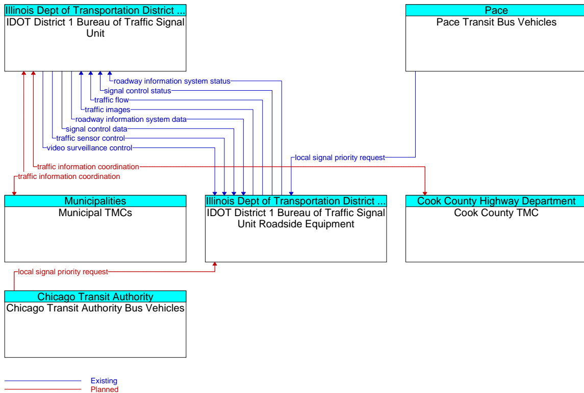
Figure A3-51: Suburban Chicago ATMS - Centralized Traffic Control (ID 44)
