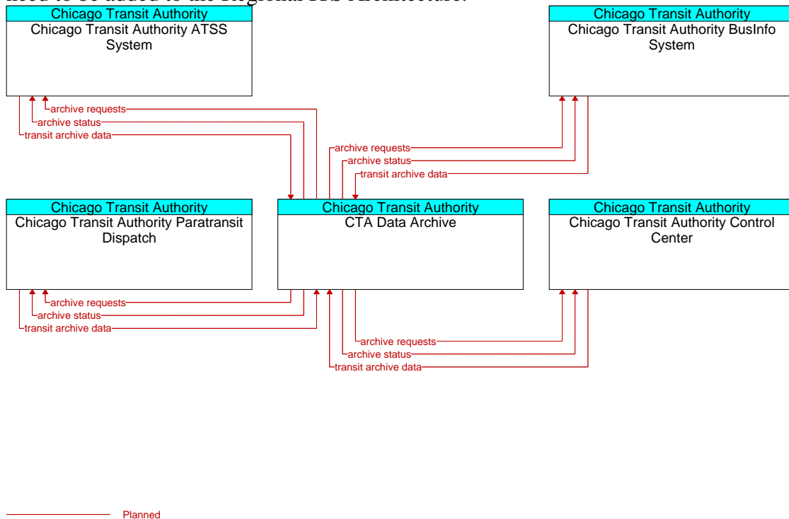
Figure A3-95: CTA Archive (ID 88)
