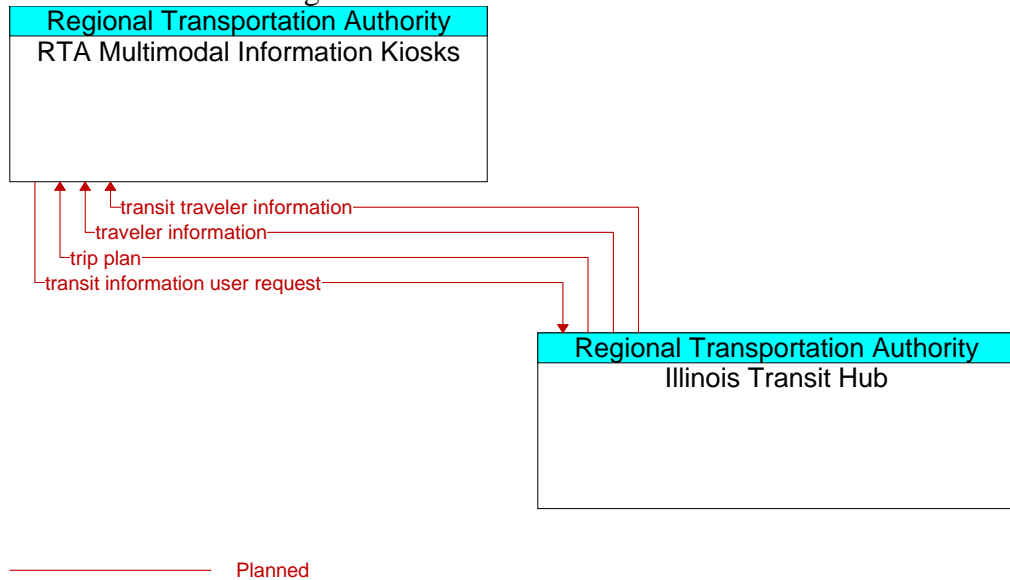
Figure A3-82: RTA Demo Projects: ATIS- Regional Traveler Info Kiosks (ID 78b)
