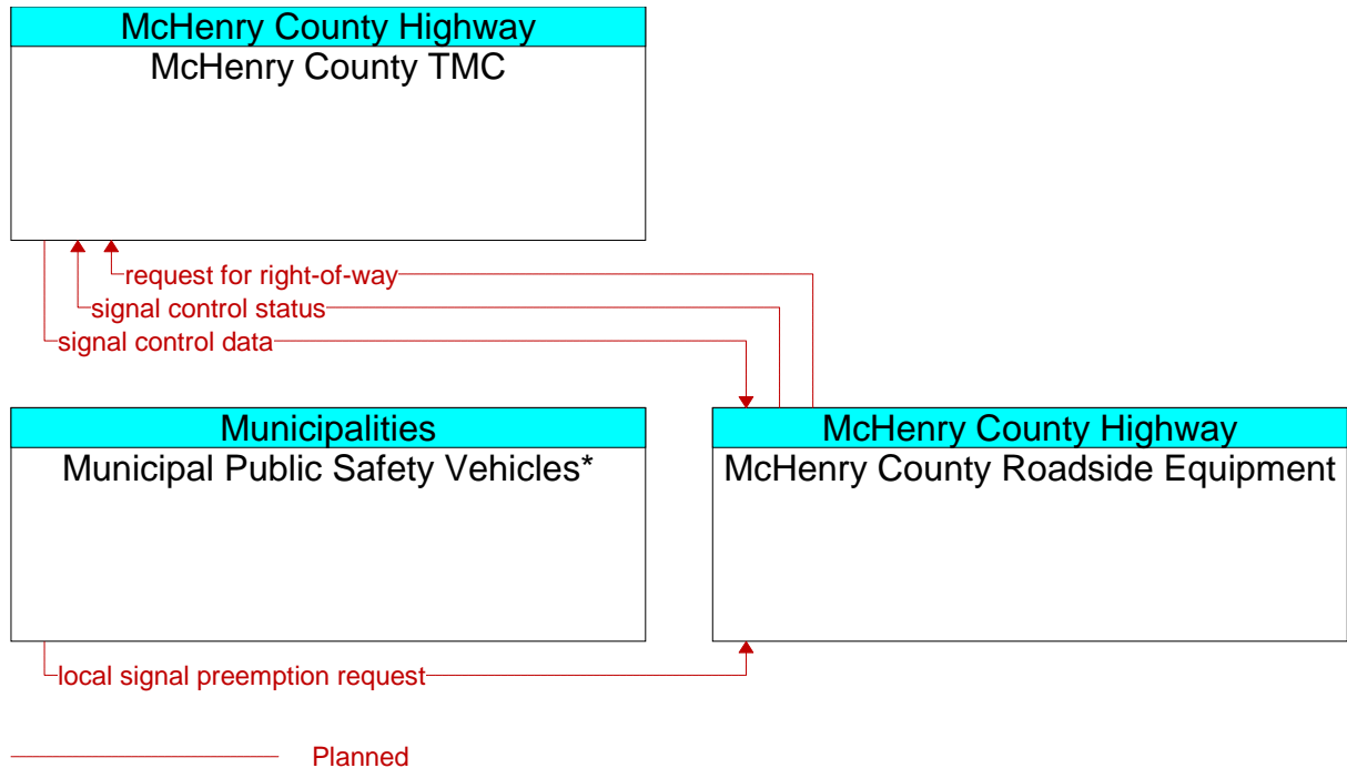
Figure A3-42: McHenry County Field Devices (ID 35)
