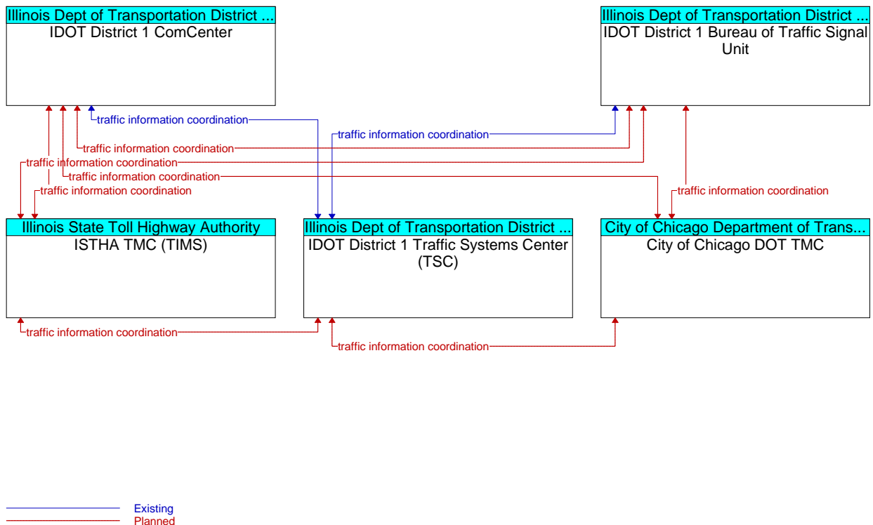
Figure A3-52: CCTV Surveillance Sharing (ID 48)
