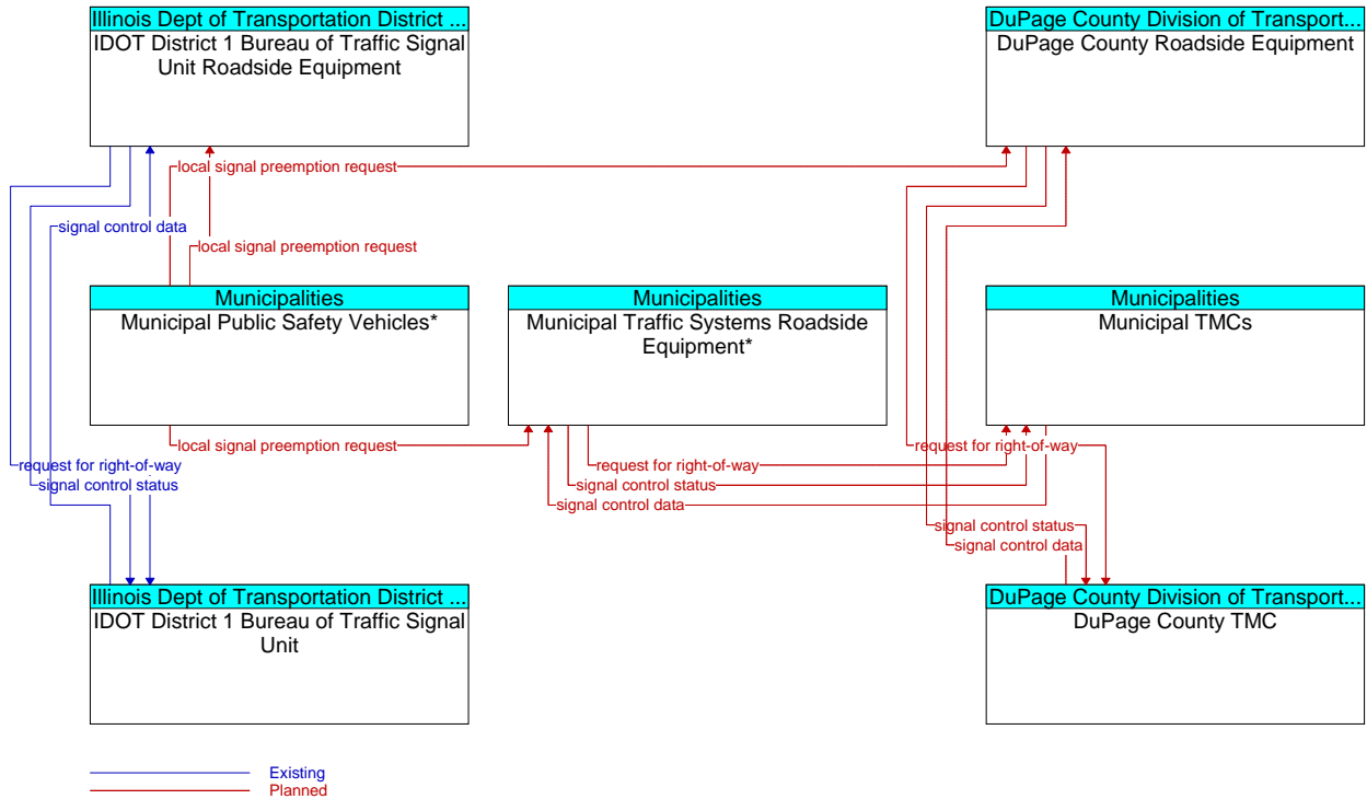
Figure A3-26: DuPage Emergency Management and Signal Preemption (ID 25)
