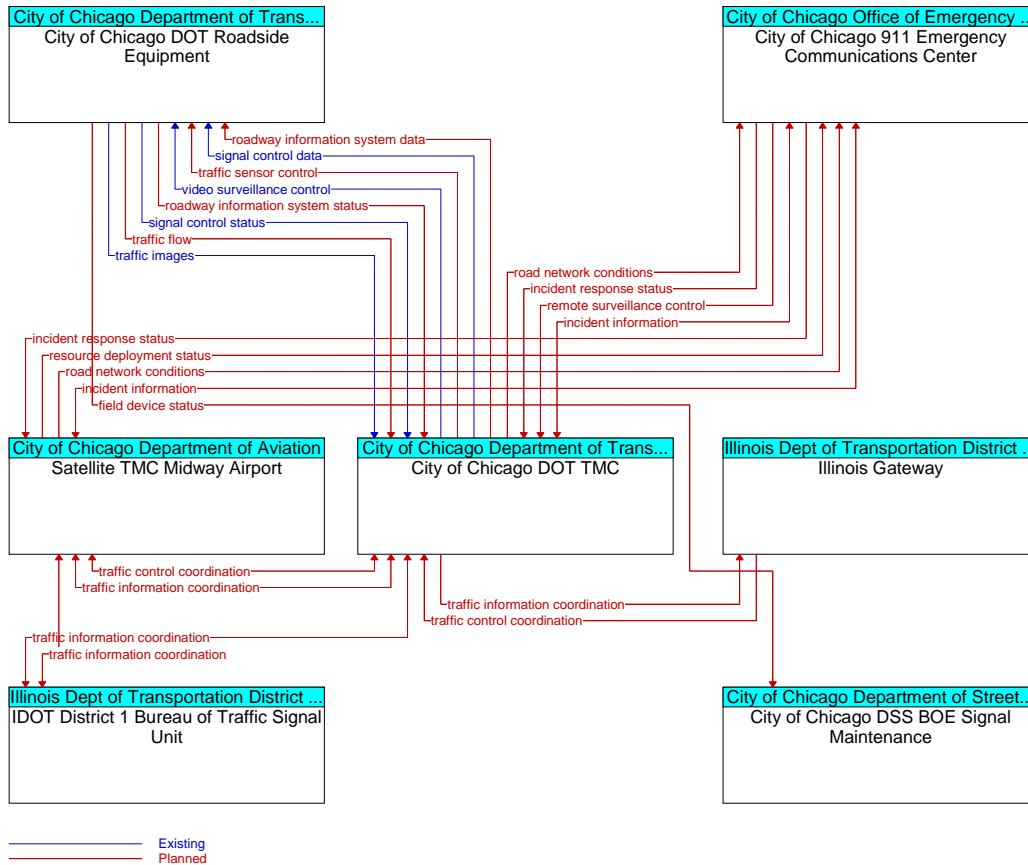
Figure A3- 5: Cicero Ave Smart Corridor ATMS Project (ID 4)
