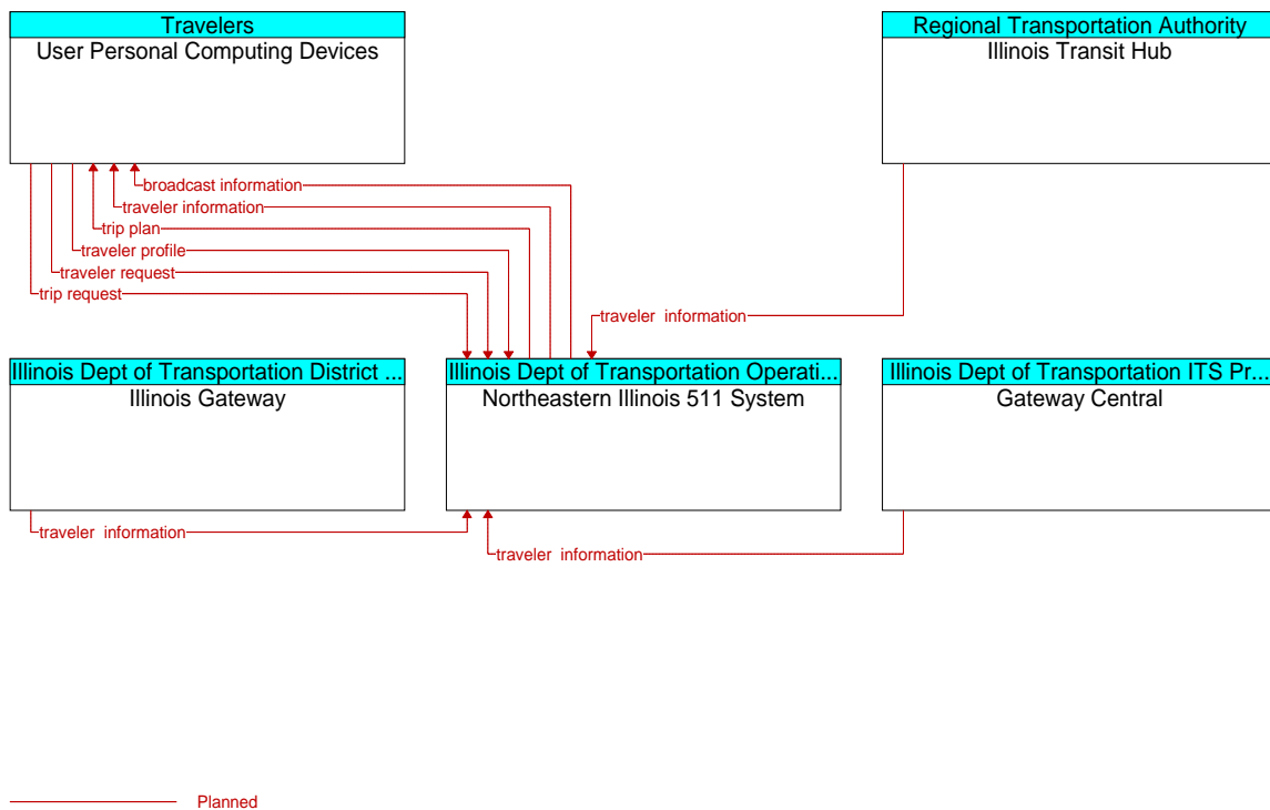
Figure A3-61: Statewide 511 Service (ID 56)
