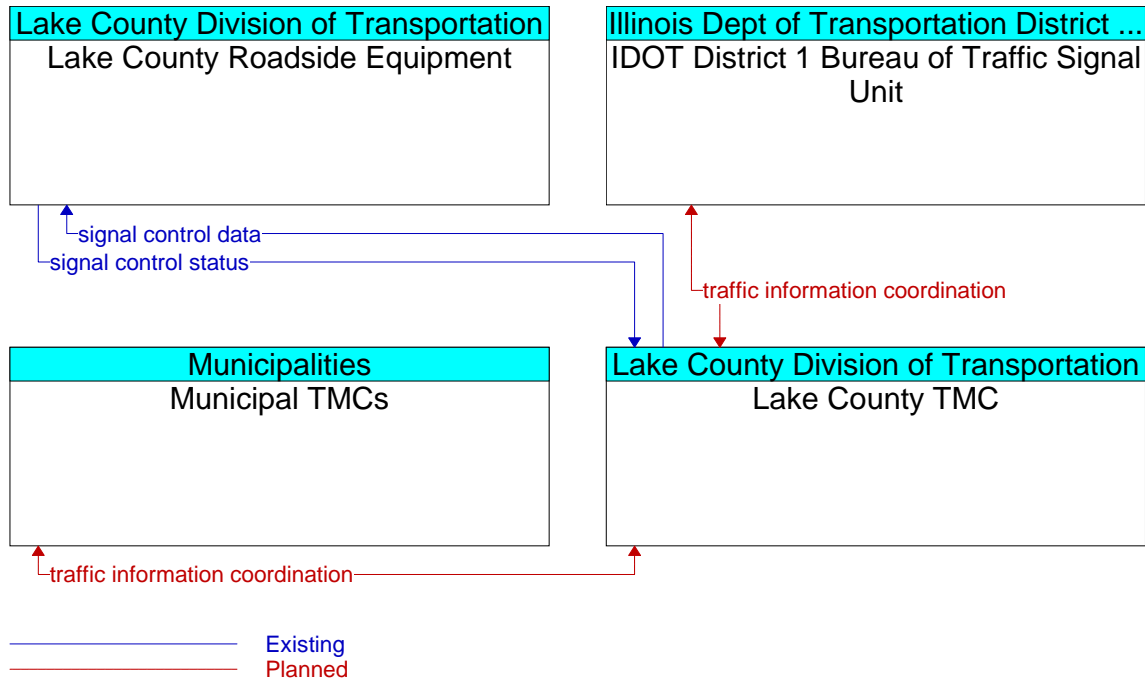
Figure A3-38: Lake County Signal Interconnects (ID 33)
