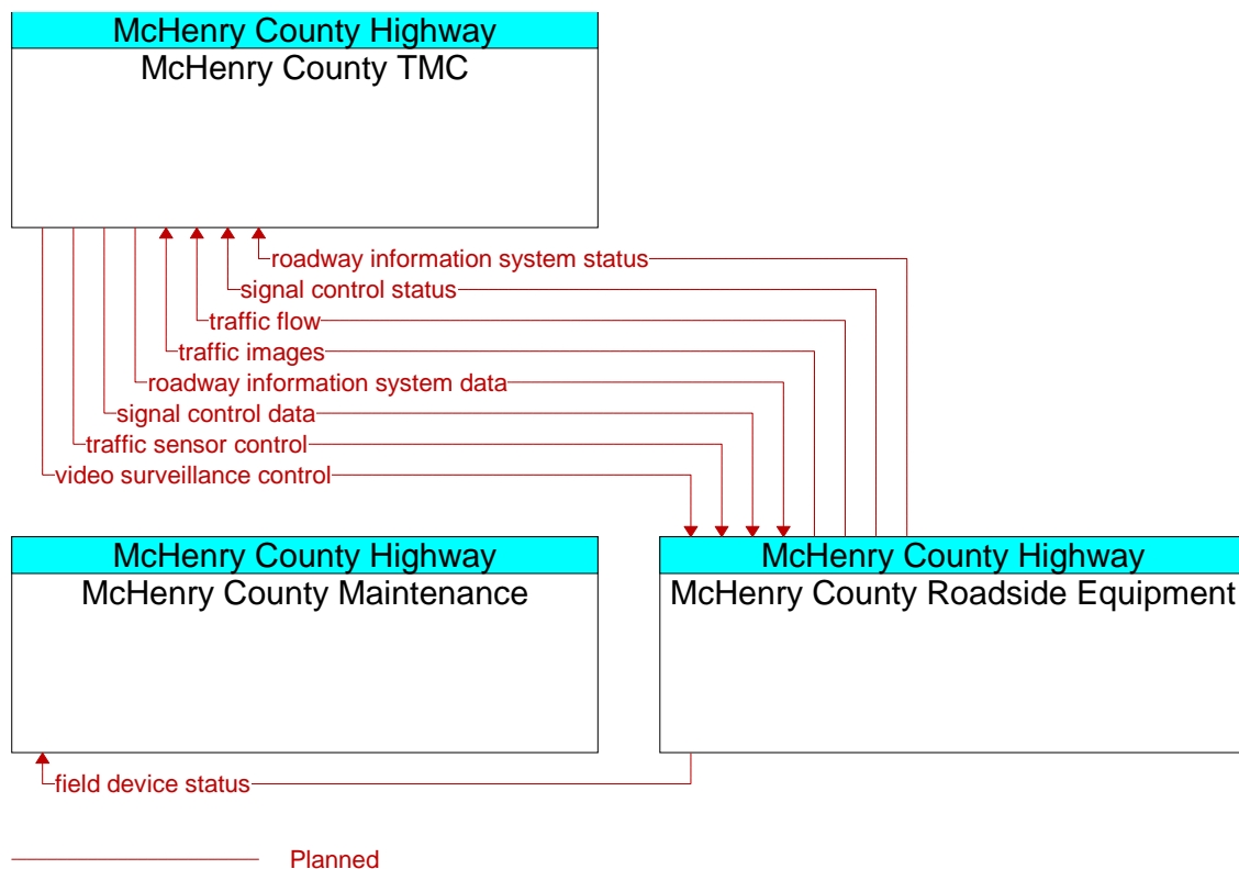
Figure A3-39: McHenry County Traffic Management Center- Roadside Interfaces (ID 34)
