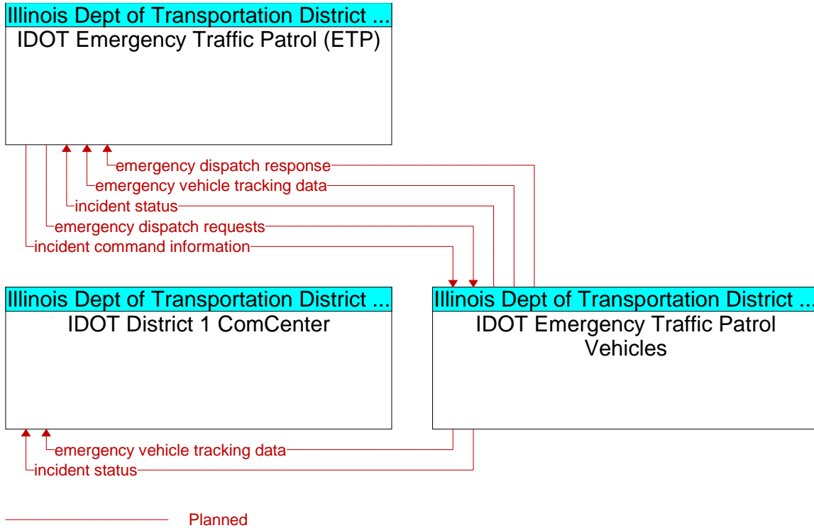
Figure A3-57: Regionwide Emergency Traffic Operations Systems (ETOS) Upgrade (ID 53)
