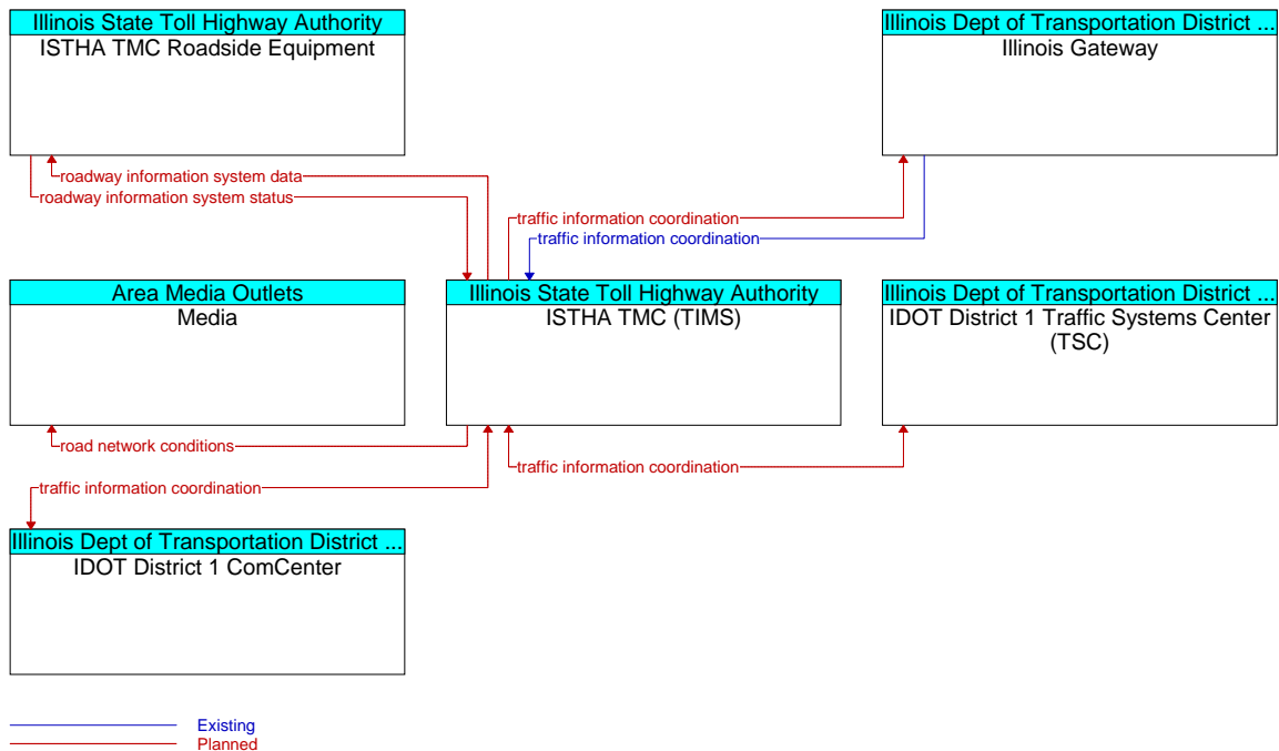
Figure A3-73: ISTHA DMS Deployment (ID 73)
