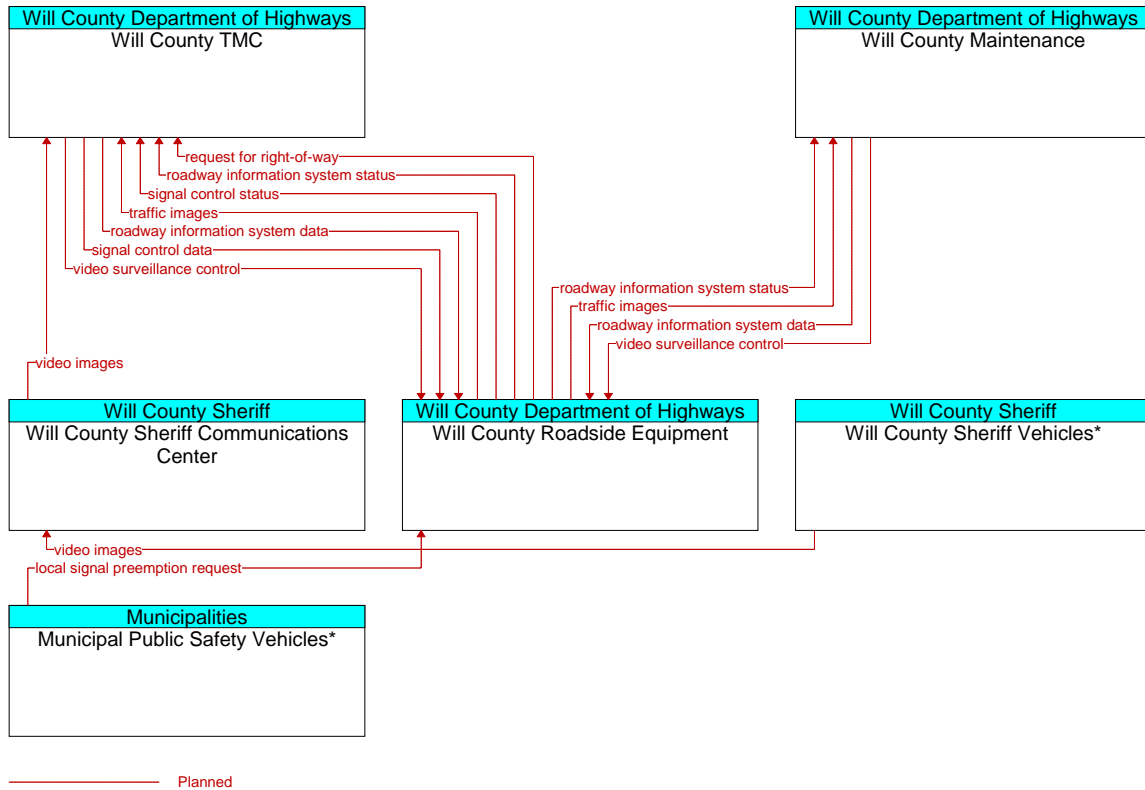
Figure A3-47: Will County Field Devices (ID 38)
