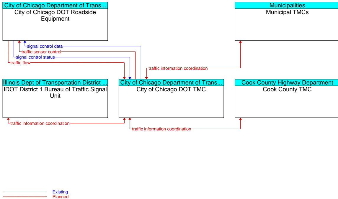
Figure A3-11: City of Chicago Interconnects
