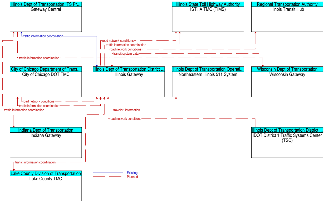
Figure A3-59: GATEWAY Traveler Information System, Phase II (ID 55)- traffic management, transit and 511 interfaces
