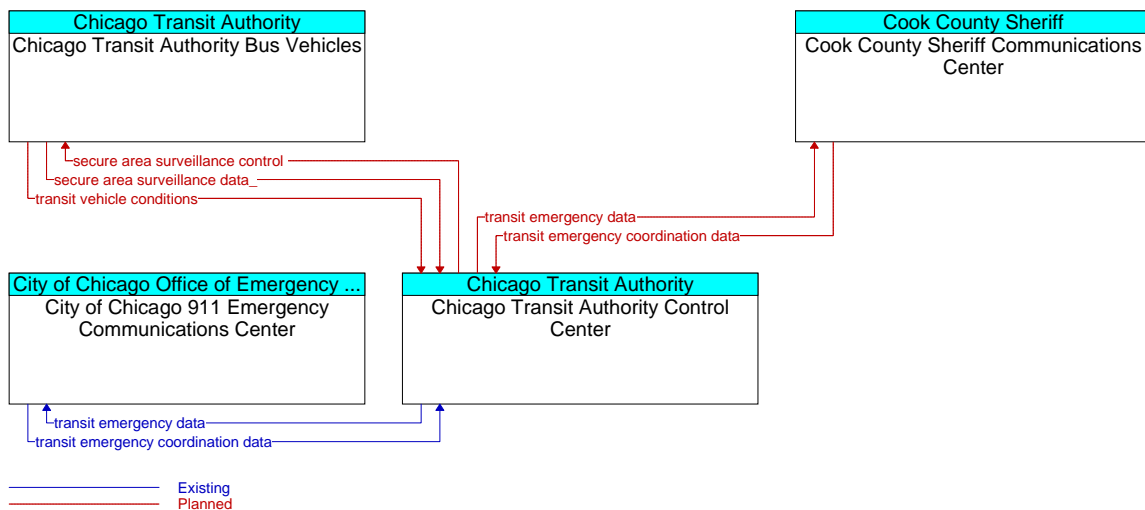
Figure A3-87: RTA Projects: Transit Vehicle Safety Projects (ID 79)
