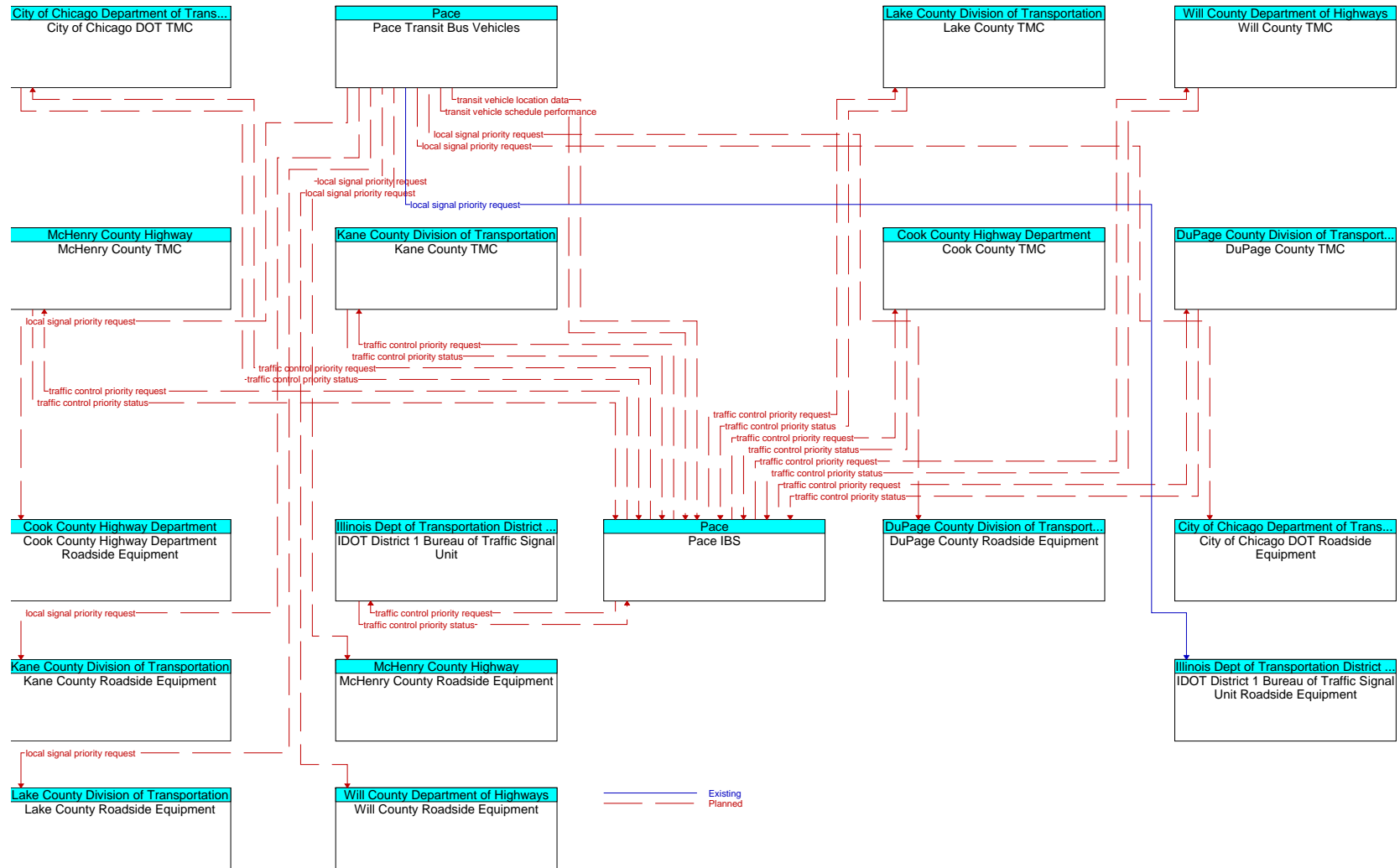
Figure A3-104: Wide Transit Signal Priority Deployment (ID 100)
