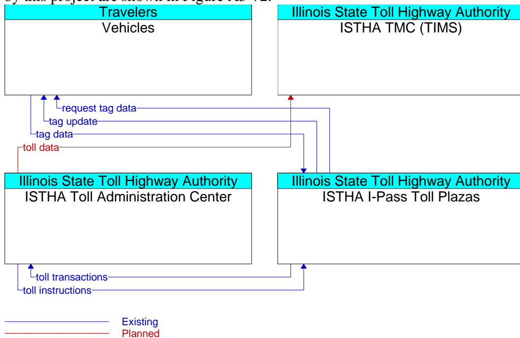
Figure A3-72: ISTHA Systemwide Open Road Tolling (ORT) (ID 72)
