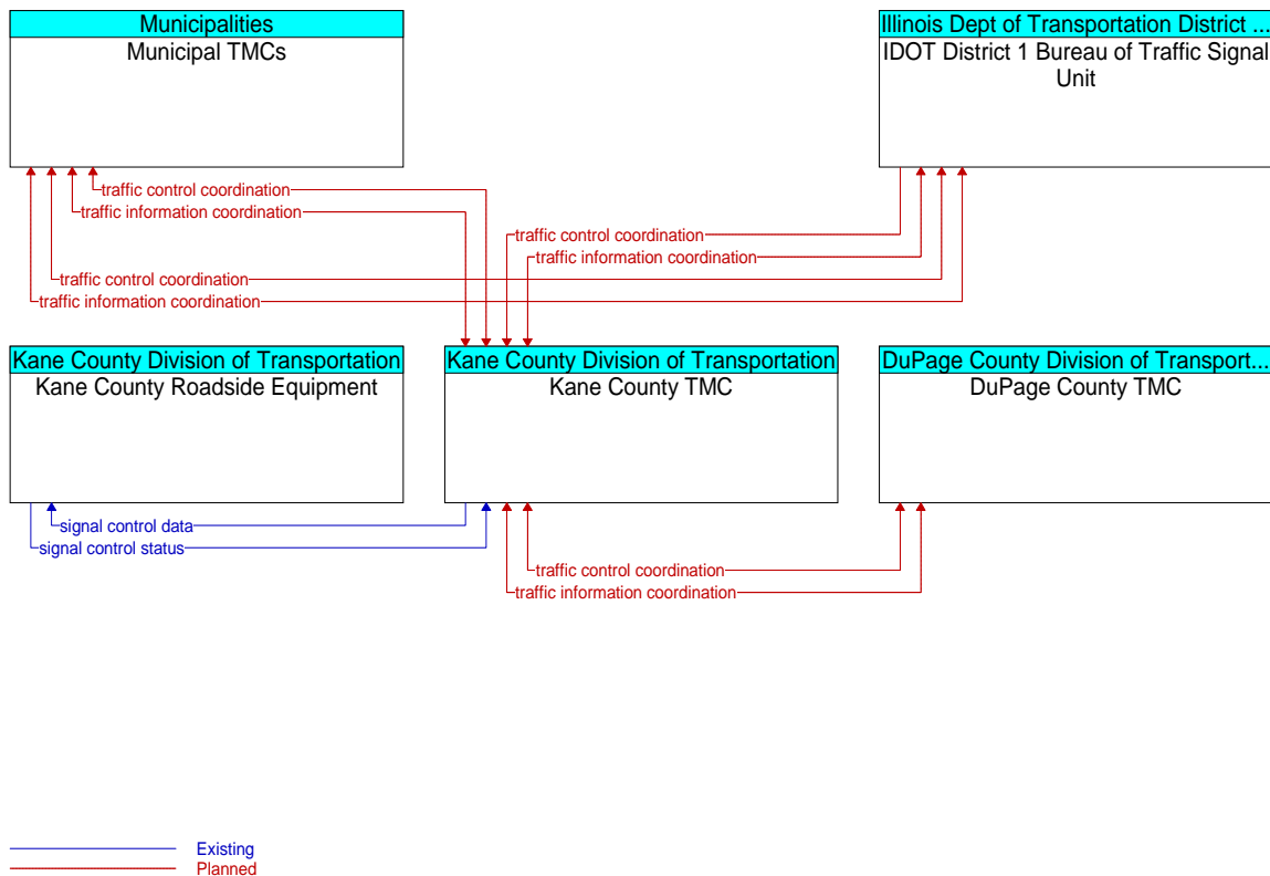
Figure A3-33: Kane County Signal Interconnects (ID 30)
