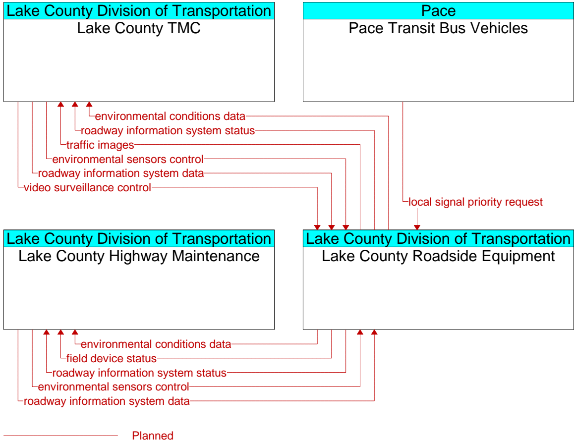
Figure A3-37: Lake County Field Devices (ID 32)
