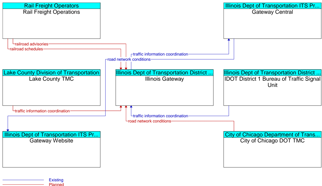
Figure A3-65: Railroad Grade Crossing Delay - Traveler Information System (ID 64)
