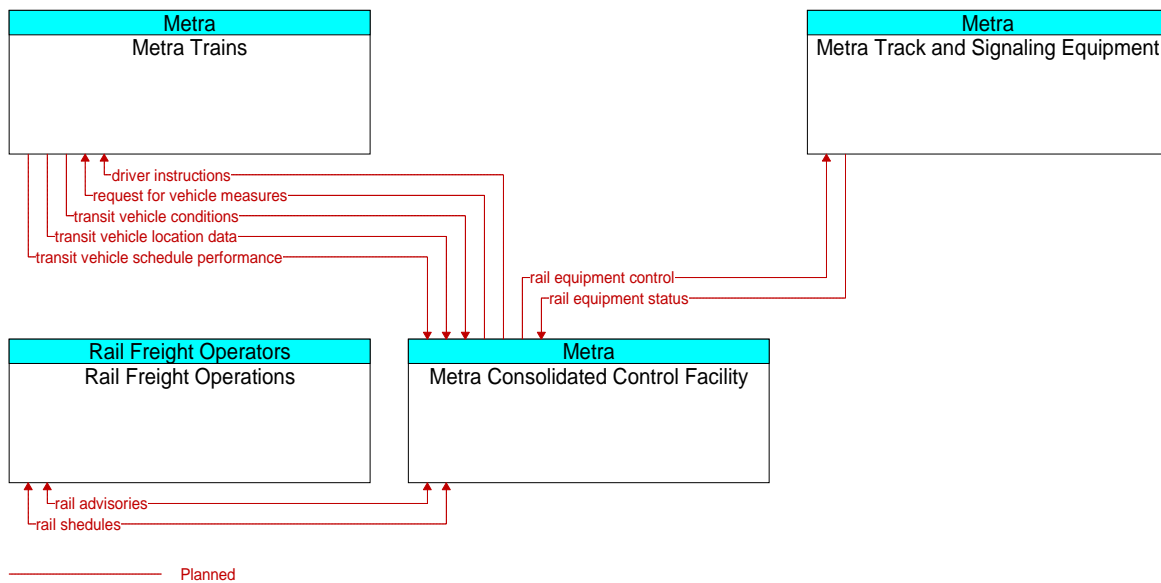
Figure A3-96: Metra Rail Dispatch & Signaling System Upgrade (ID 89)
