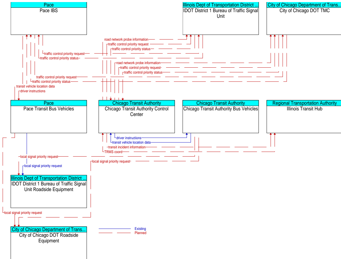
Figure A3-79: RTA Demo Projects- APTS (ID 76)
