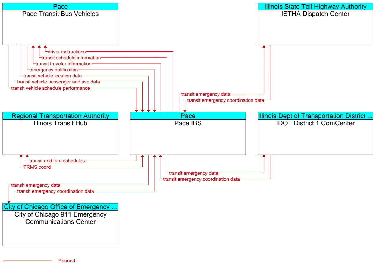
Figure A3-100: Pace Intelligent Bus System (ID 94)
