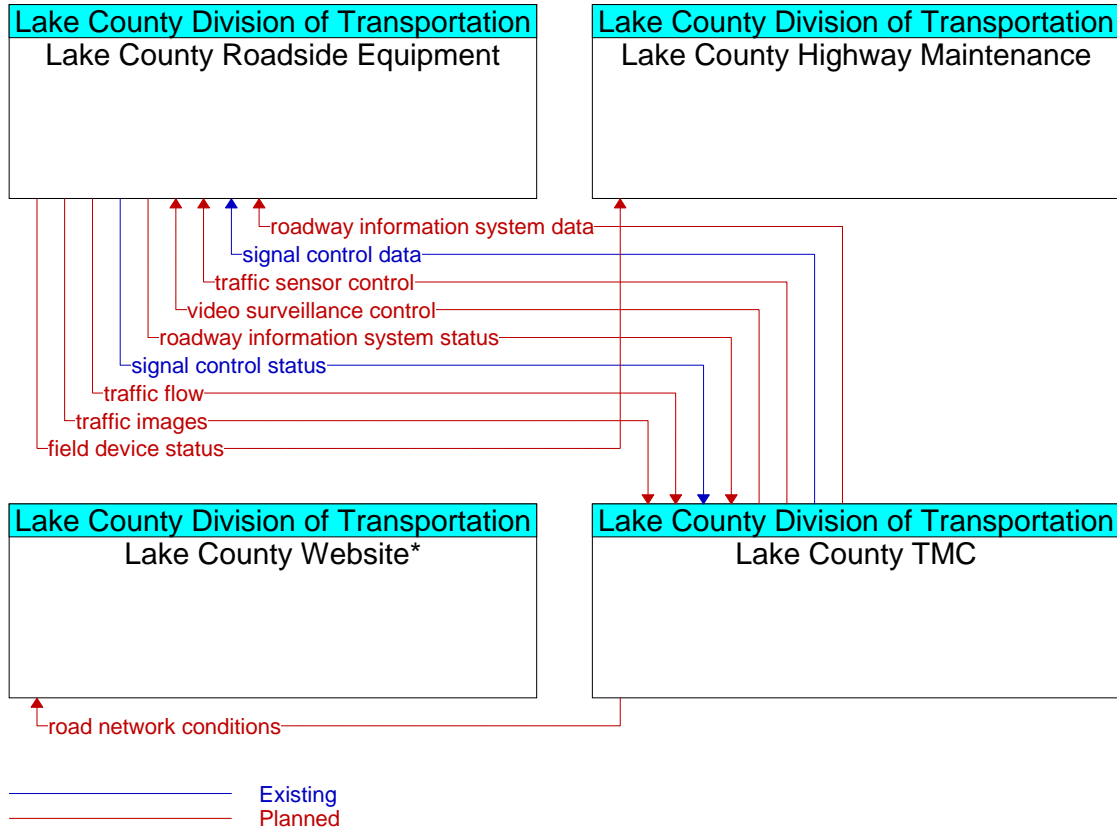
Figure A3-34: Lake County Traffic Management Center- Roadside Interfaces (ID 31)
