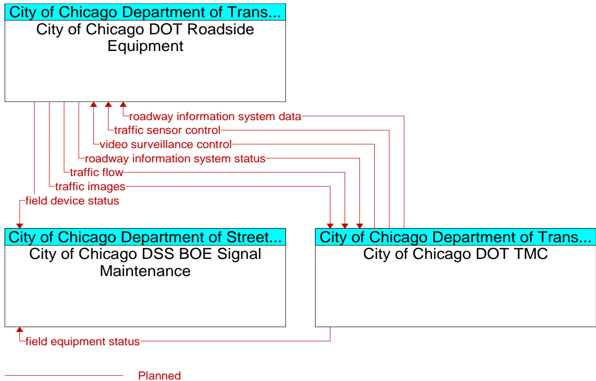
Figure A3-14: US 41 Lake Shore Drive information system (ID 14)
