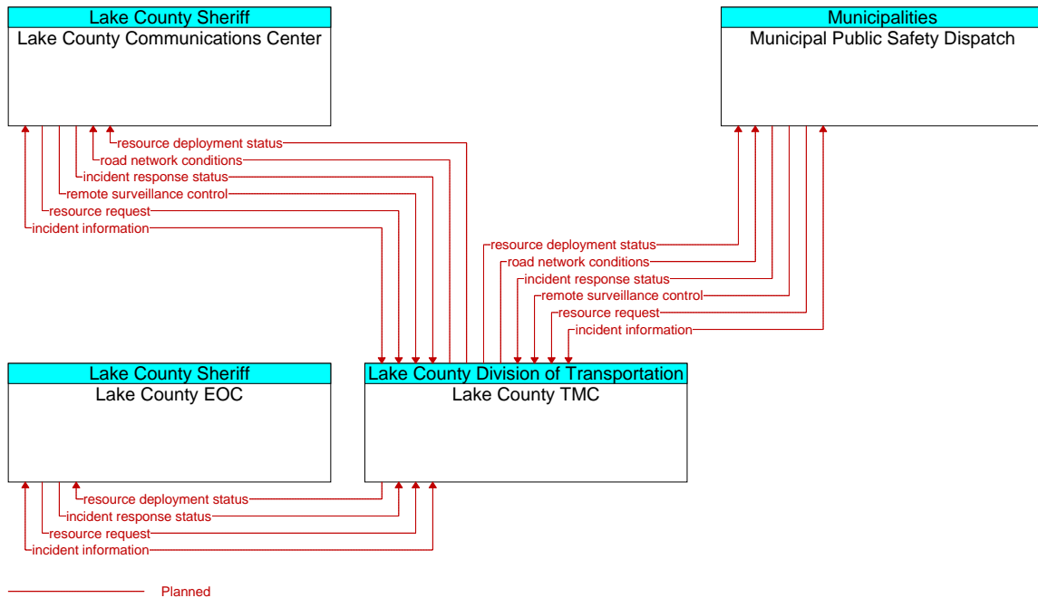
Figure A3-36: Lake County Traffic Management Center- Emergency Management Interfaces (ID 31)
