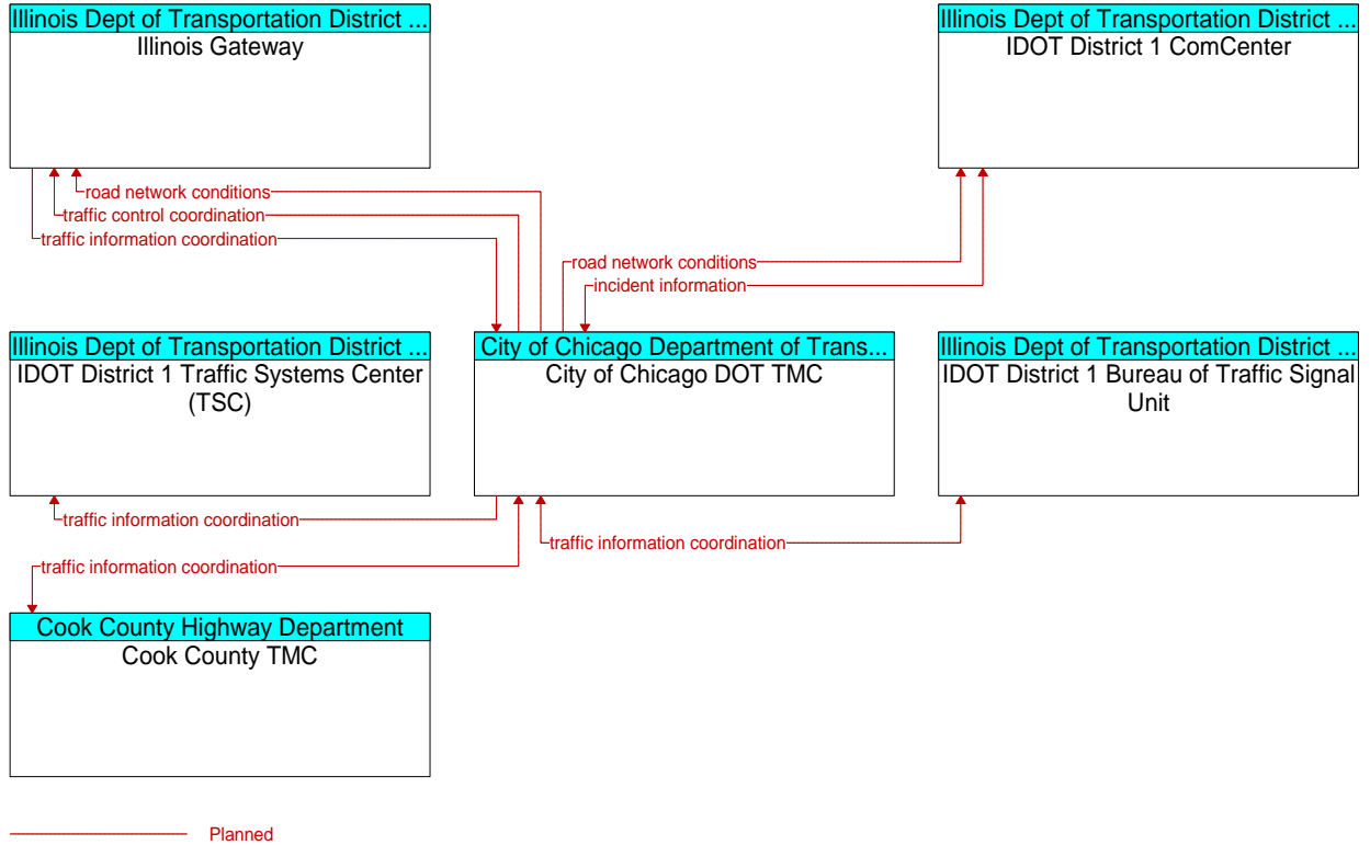
Figure A3-2: Development of Chicago TMC (ID 2)- Traffic Management Interfaces
