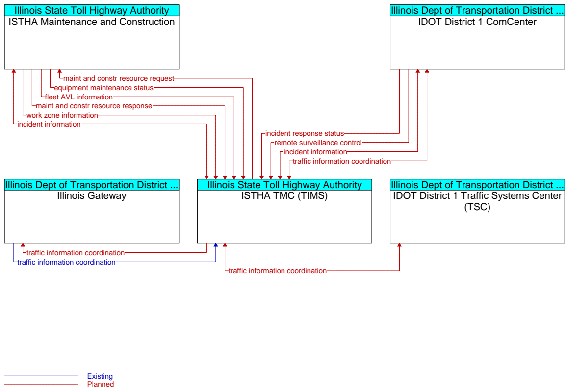
Figure A3-69: ISTHA TIMS Enhancement (ID 69)
