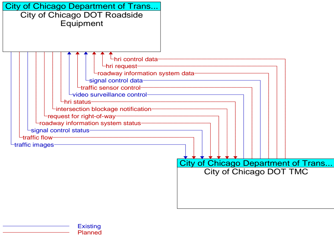
Figure A3-1: Development of Chicago TMC (ID 2)- Roadside Interface
