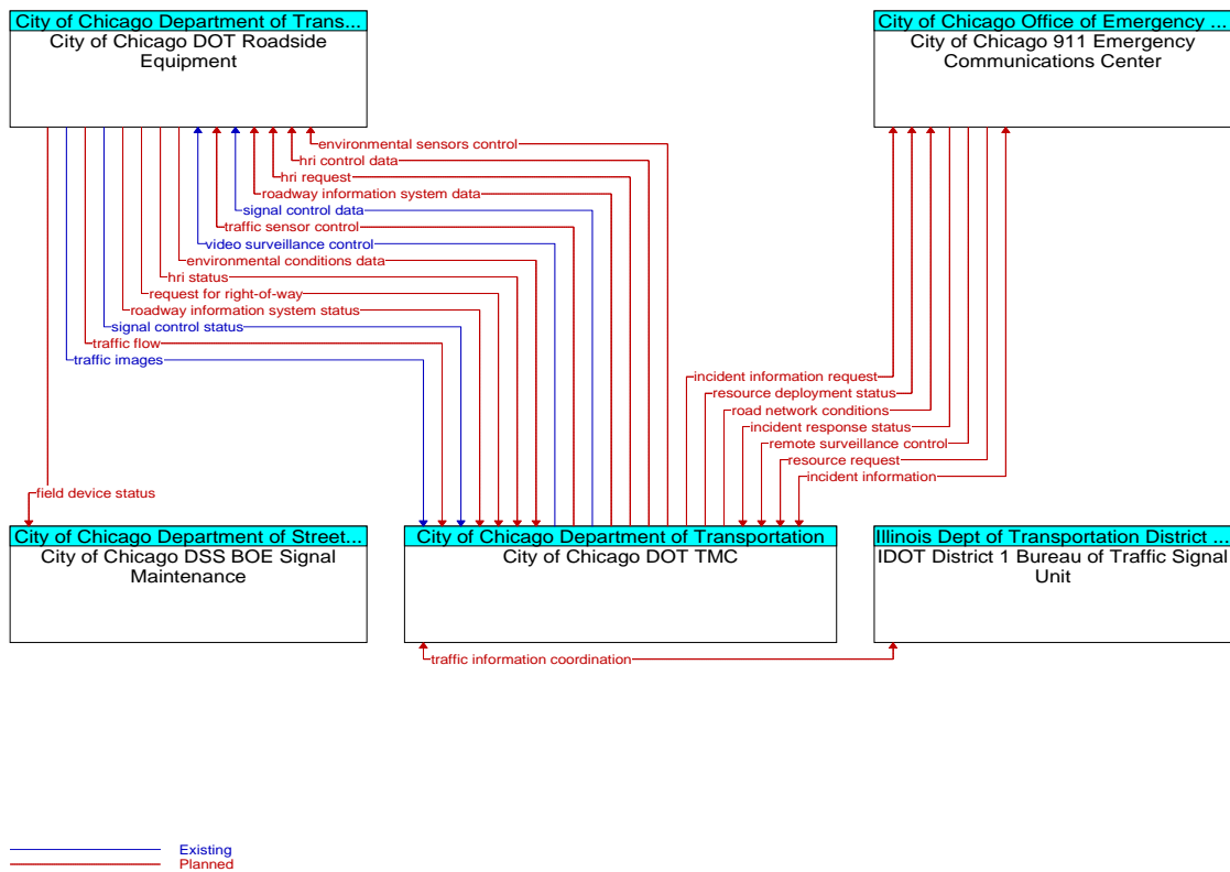
Figure A3- 7: CDOT Smart Corridors: Pulaski Road, etc. (ID 6)
