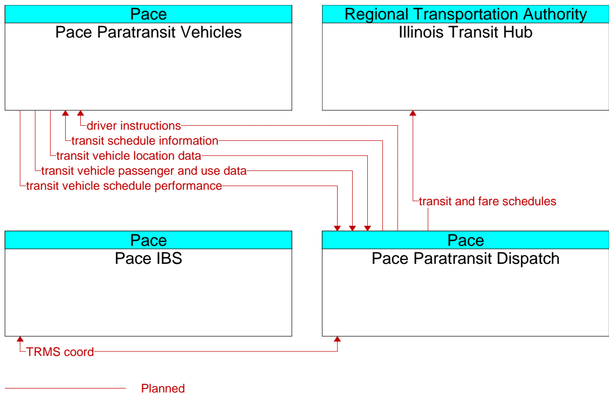
Figure A3-101: Pace Paratransit MDT/AVL (ID 95)
