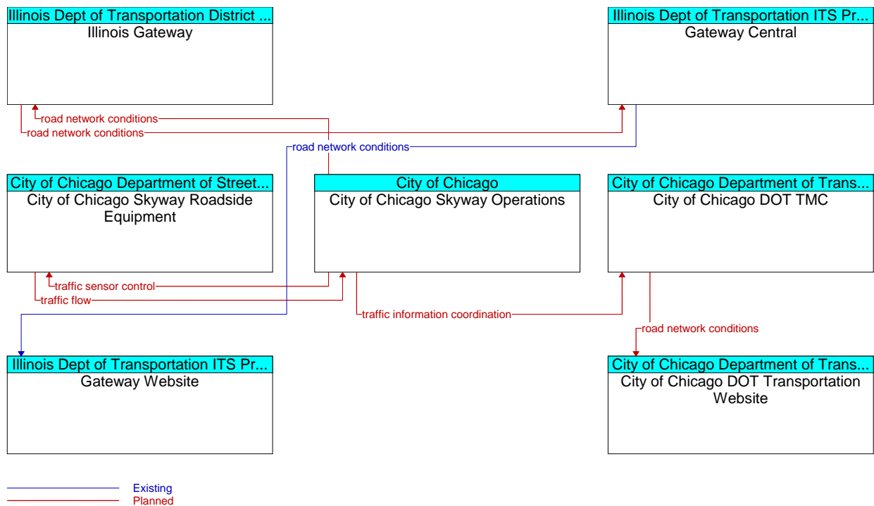
Figure A3-13: Chicago Skyway Travel Monitoring and Integration with IDOT Gateway (ID 13)
