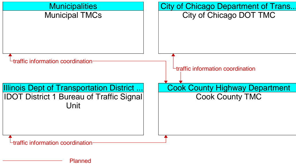
Figure A3-25: Interagency Signal Coordination- Cook County (ID 23)
