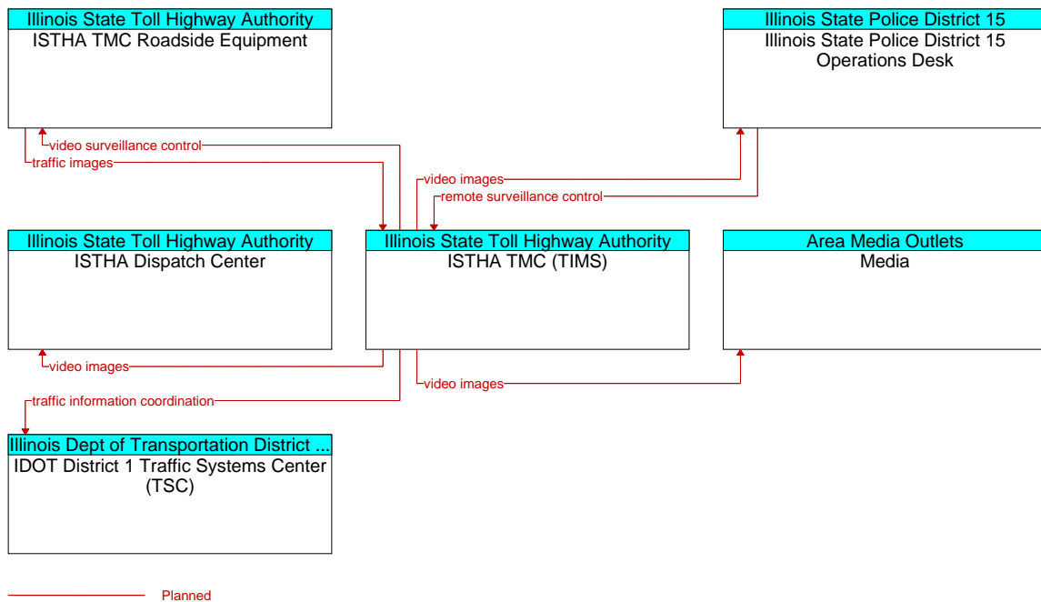
Figure A3-71: ISTHA CCTV Coverage (ID 71)
