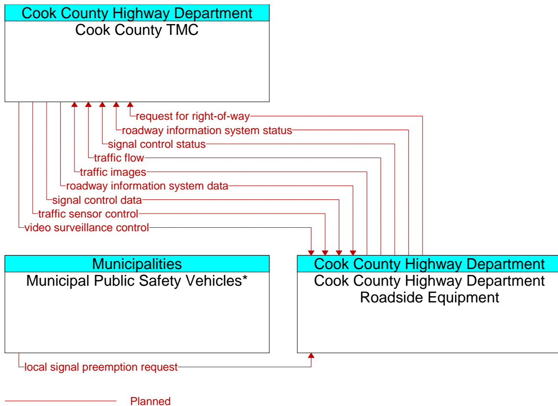
Figure A3-23: Cook County Field Devices (ID 21)
